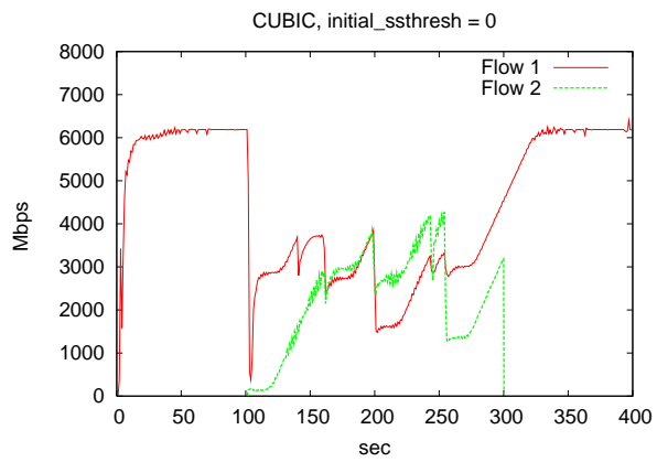
Figure 3: CUBIC, initial-ssthresh = 0
