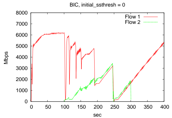
Figure 2: BIC, initial-ssthresh = 0
