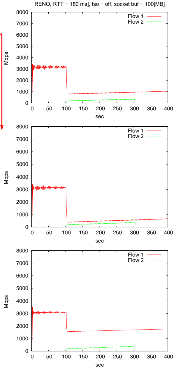
Figure 2: RENO
