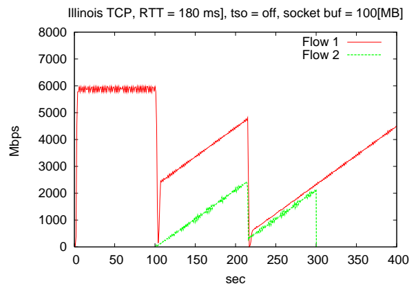
Figure 8: Illinois TCP
