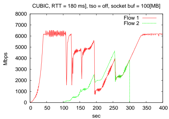
Figure 5: CUBIC
