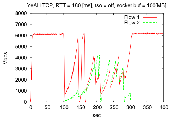
Figure 7: YeAH TCP
