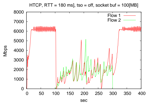
Figure 6: HTCP
