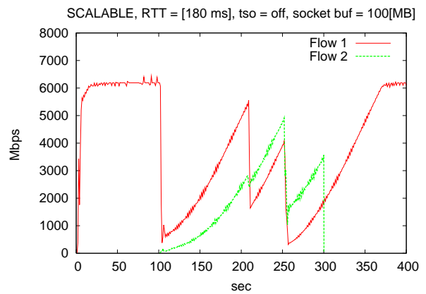
Figure 4: SCALABLE TCP
