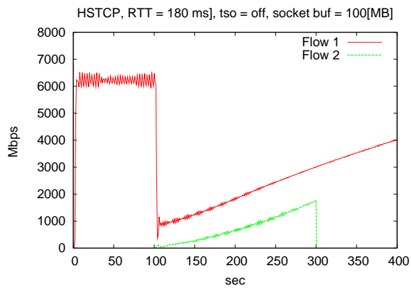
Figure 3: HSTCP
