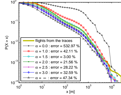
Fig. 5. Flight distributions obtained from LATP for different \alpha values performed on top of waypoints extracted from the KAIST traces and the percentage difference between the sum of flights generated from LATP and that of flights from real traces
